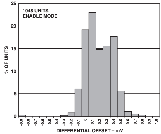
TPC 10. Differential Input Offset Histogram
