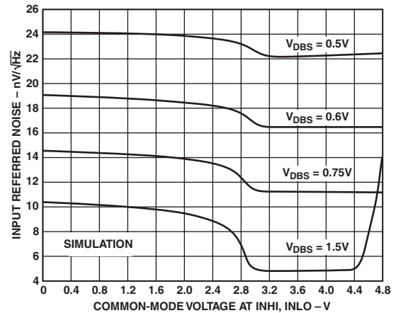
Figure 13. Input Noise vs. Common-Mode Input Voltage for V_{DBS} = 0.5\text{ V} , 0.6\text{ V} , 0.75\text{ V} , and 1.5\text{ V}
