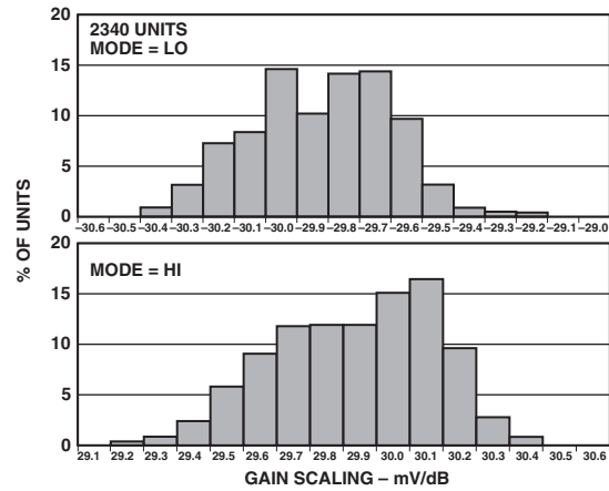
TPC 5. Gain Slope Histogram
